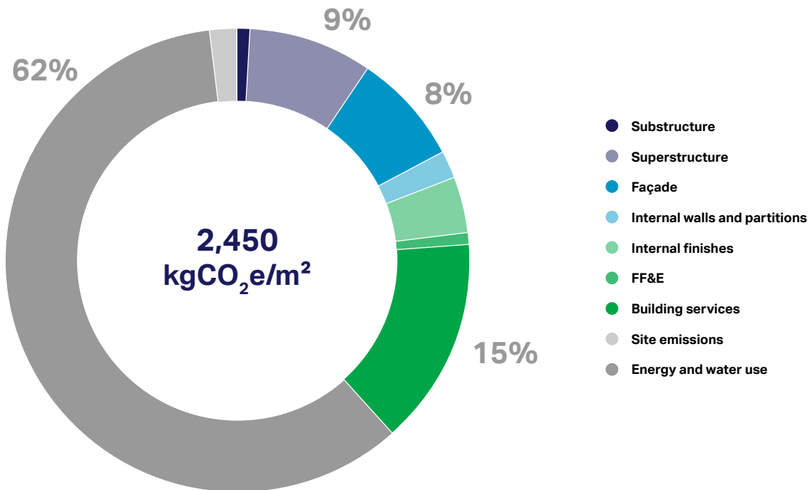
Figure 57: Whole life carbon (A-C)
