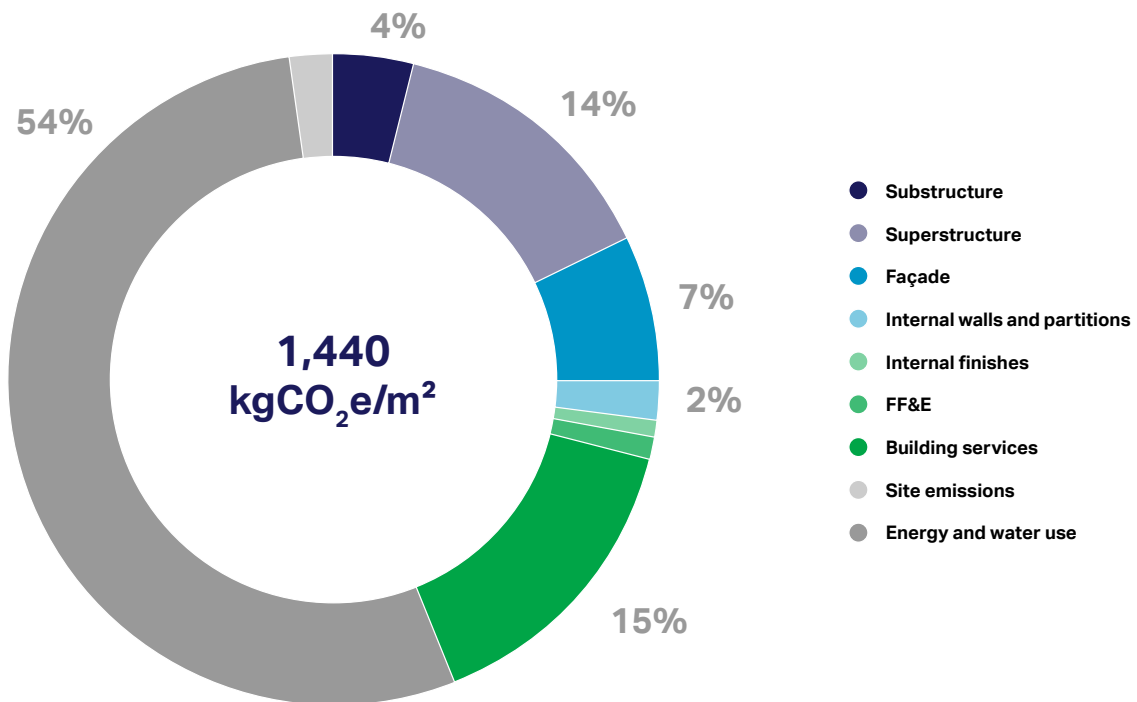
Figure 95: Whole life carbon (A-C)
