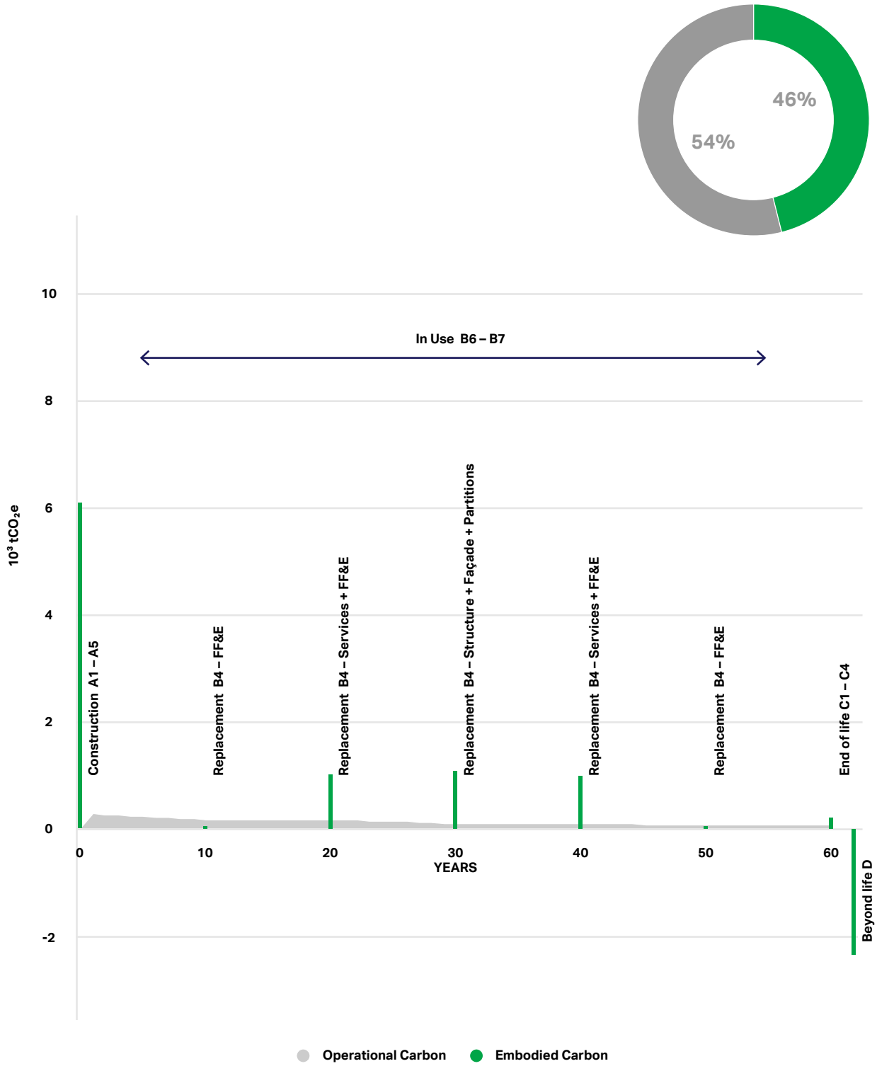
Figure 97: Whole life carbon emissions
