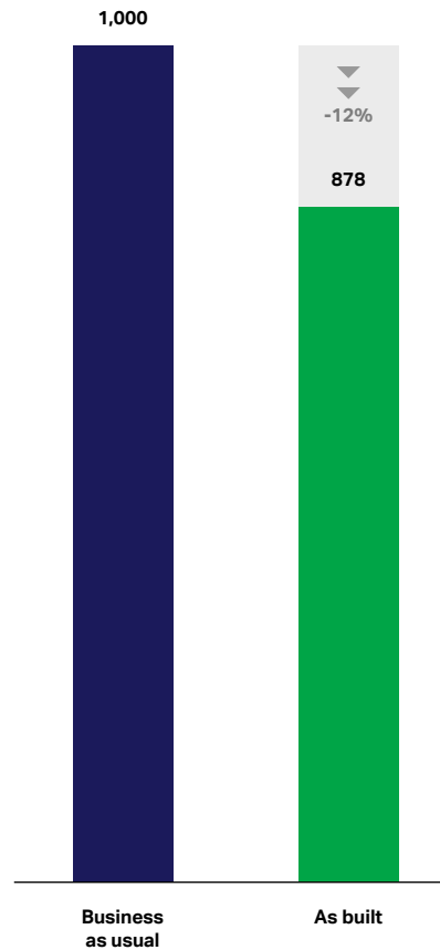
Figure 88: Carbon emissions at practical completion (kgCO 2 e/m 2 GIA)
