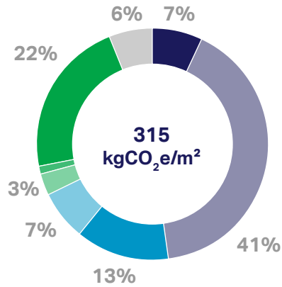
Figure 24: Embodied carbon at practical completion (A1-A5)
