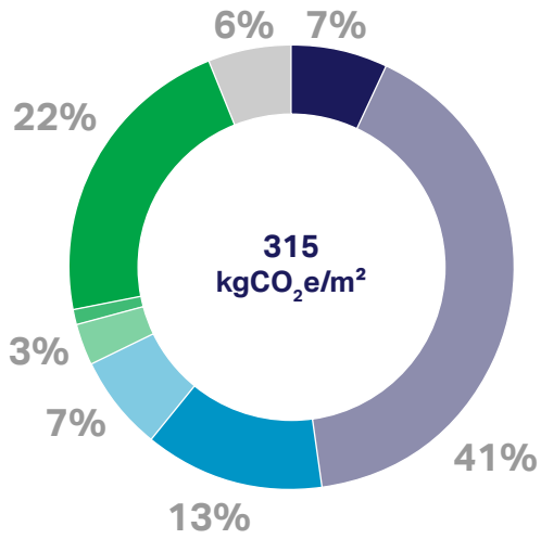
Figure 77: Embodied carbon at practical completion (A1-A5)
