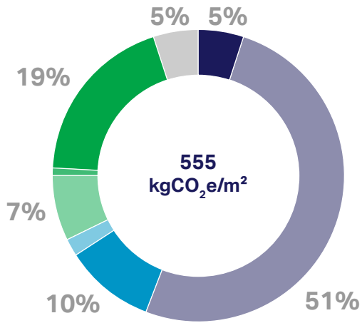
Figure 69: Embodied carbon at practical completion (A1-A5)
