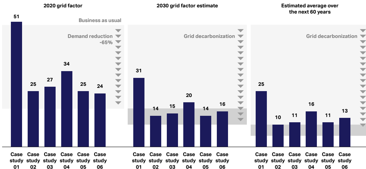
Figure 39: Operational carbon – kgCO 2 e / m 2 / year
