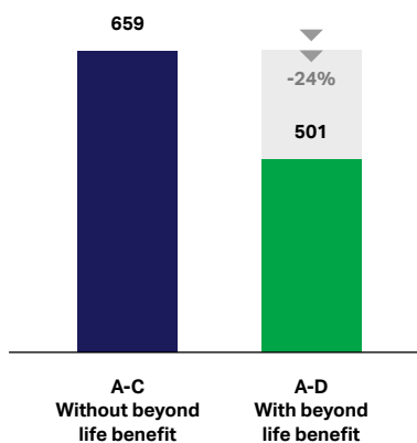
Figure 51: Whole life embodied carbon results (kgCO 2 e/m 2 )
