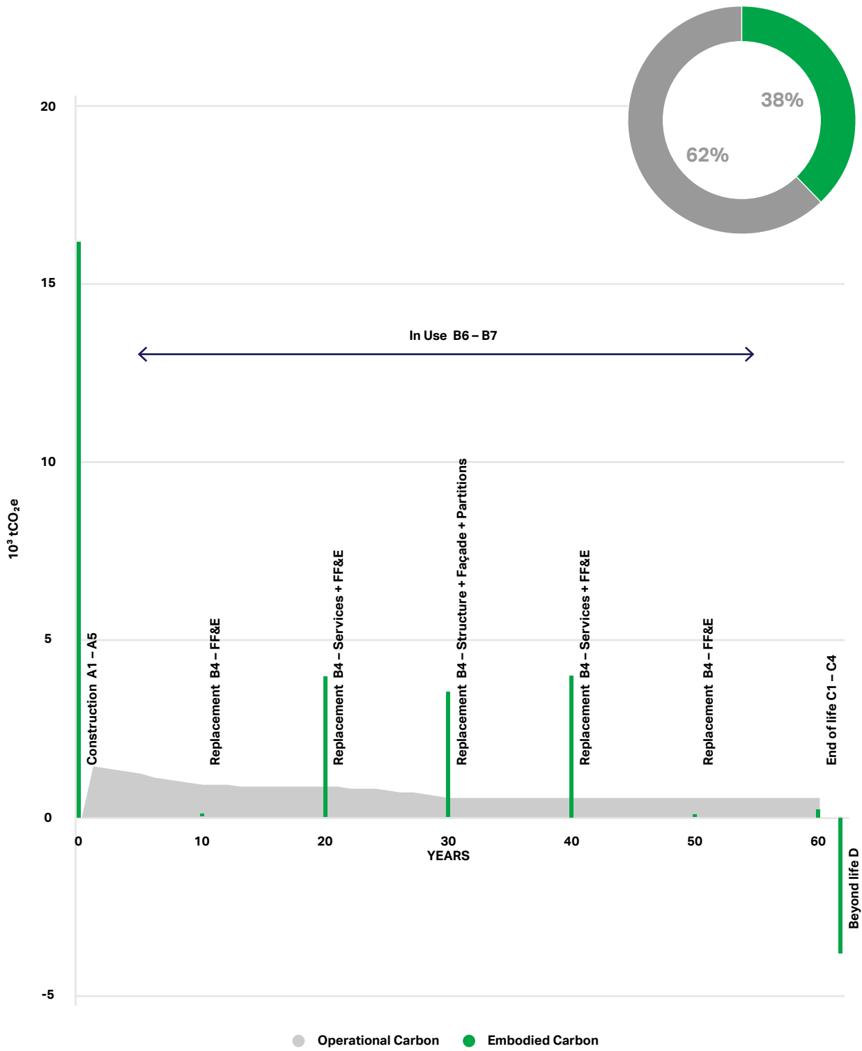
Figure 59: Whole life carbon emissions
