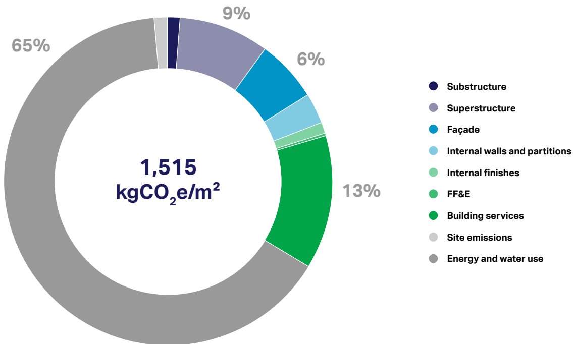
Figure 79: Whole life carbon (A-C)
