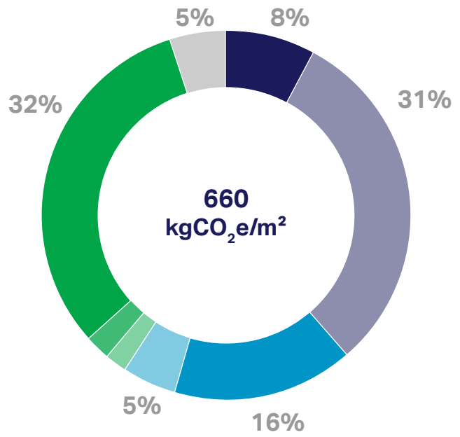
Figure 94: Embodied carbon over the life cycle (A-C)
