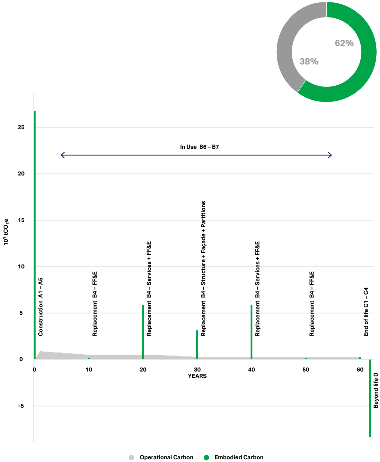
Figure 66: Whole life carbon emissions
