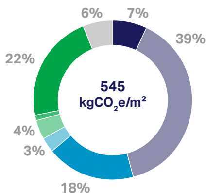
Figure 15: Embodied carbon at practical completion (A1-A5)
