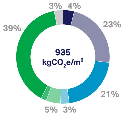
Figure 16: Embodied carbon over the life cycle (A-C)
