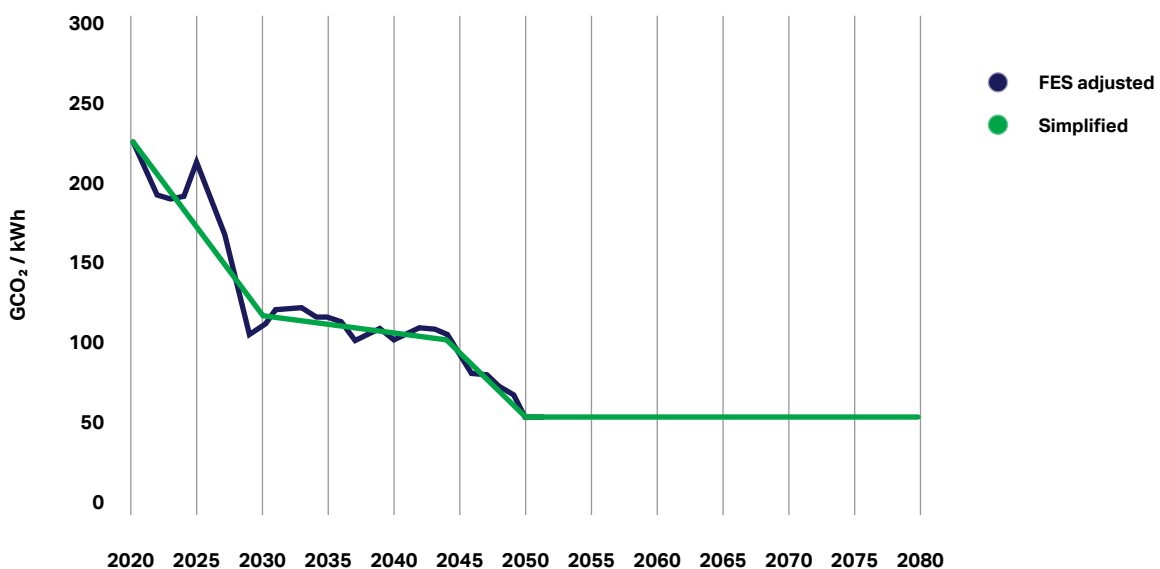
Figure 8: CO 2 intensity of electricity generation – estimated progression
