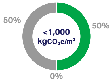
Figure 42: Whole life carbon (A-C) aspirational performance by 2030
