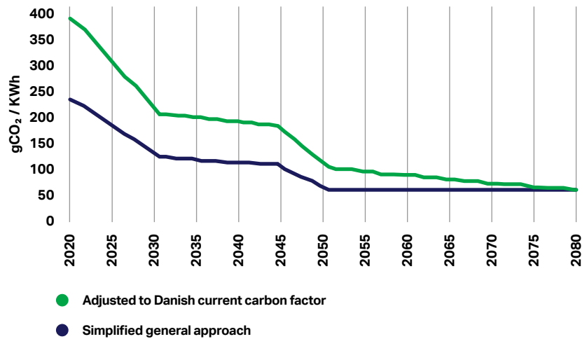
Figure 84: CO 2 intensity of electricity generation – estimated progression
