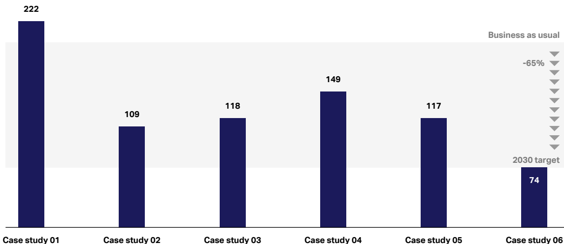
Figure 38: Energy use intensity (kWh / m 2 / year)
