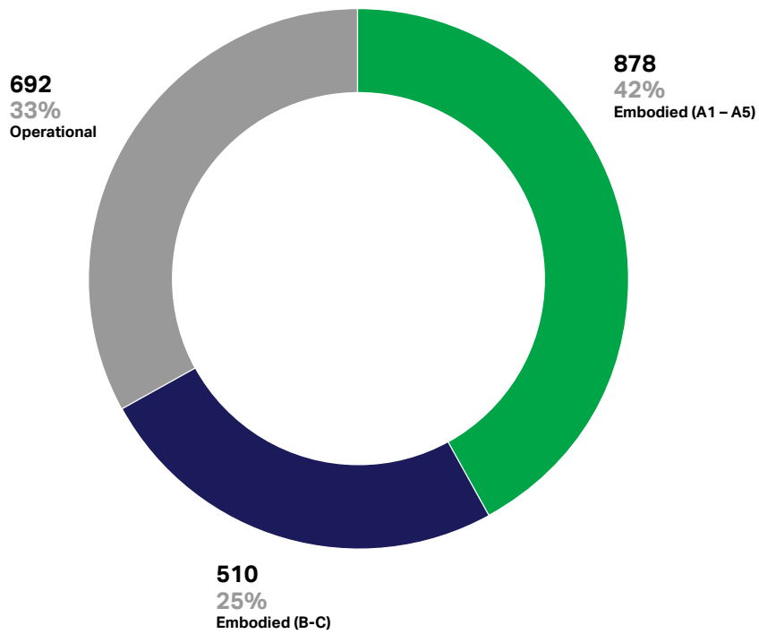
Figure 90: WLCA summary (kgCO 2 e/m 2 )
