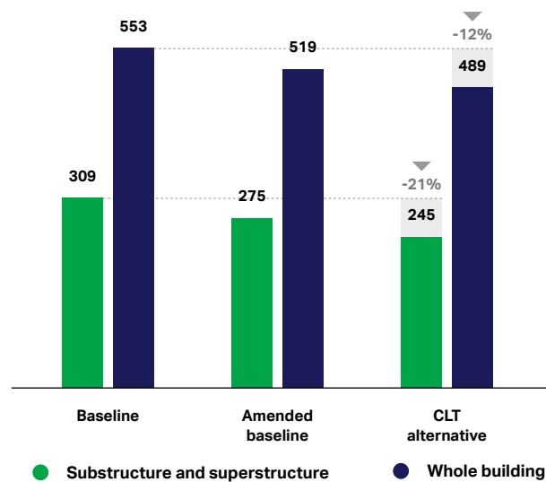
Figure 73: Potential embodied carbon reductions A1-A4 (kgCO 2 e/m 2 GIA)
