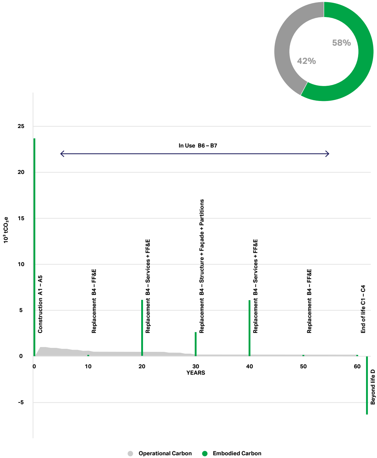
Figure 74: Whole life carbon emissions
