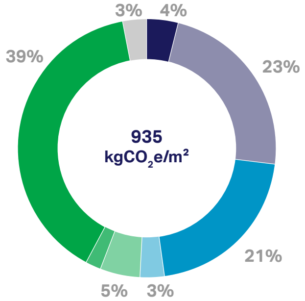
Figure 56: Embodied carbon over the life cycle (A-C)
