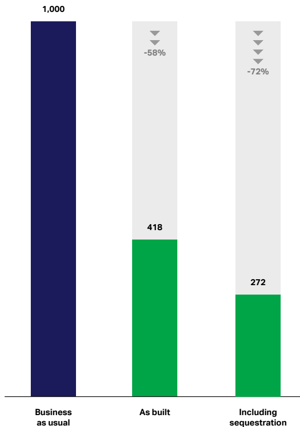
Figure 96: Carbon emissions at practical completion (kgCO 2 e/m 2 GIA)
