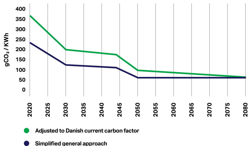
Figure 92: CO 2 intensity of electricity generation estimated progression
