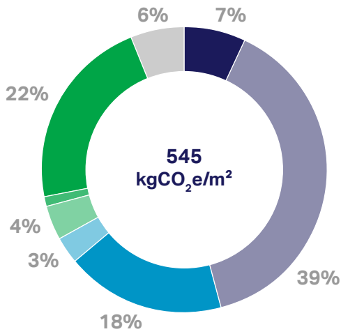
Figure 55: Embodied carbon at practical completion (A1-A5)
