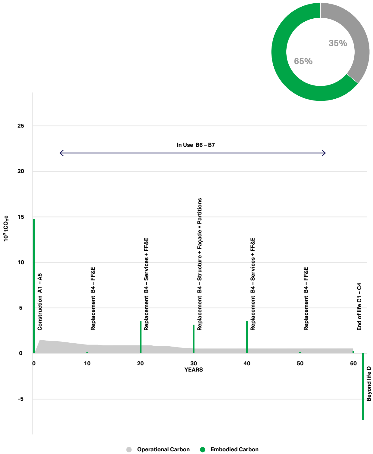
Figure 81: Whole life carbon emissions
