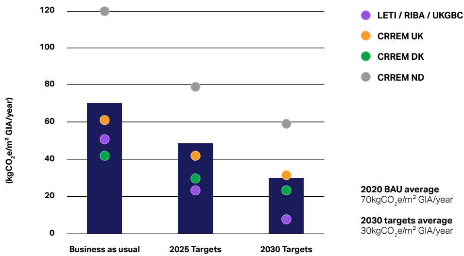
Figure 13: Operational carbon targets
