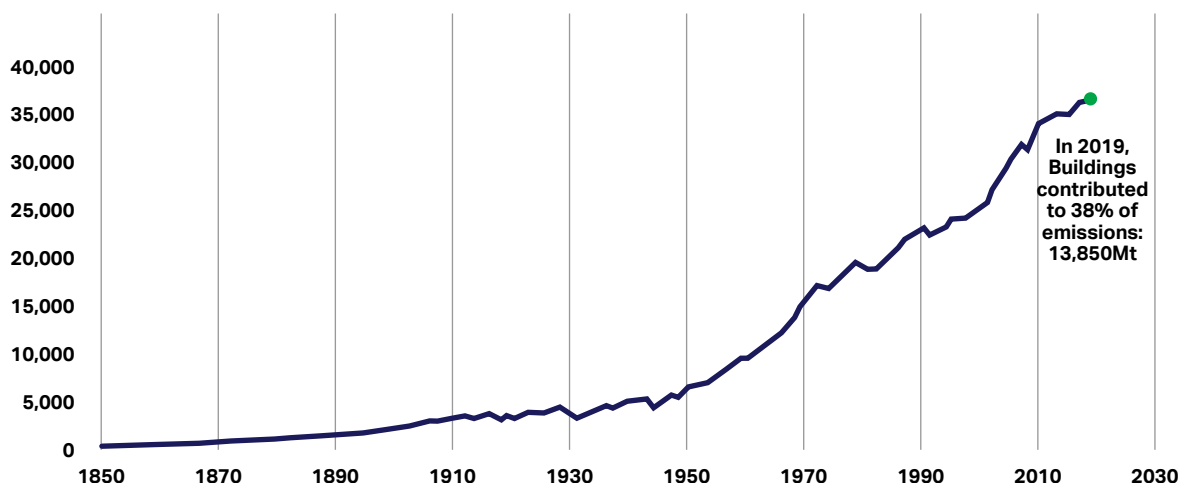
Figure 3: Global Annual CO 2 Emissions (Mt), Our World in Data and Global ABC/IEA/UNEP (2020) 3,6
