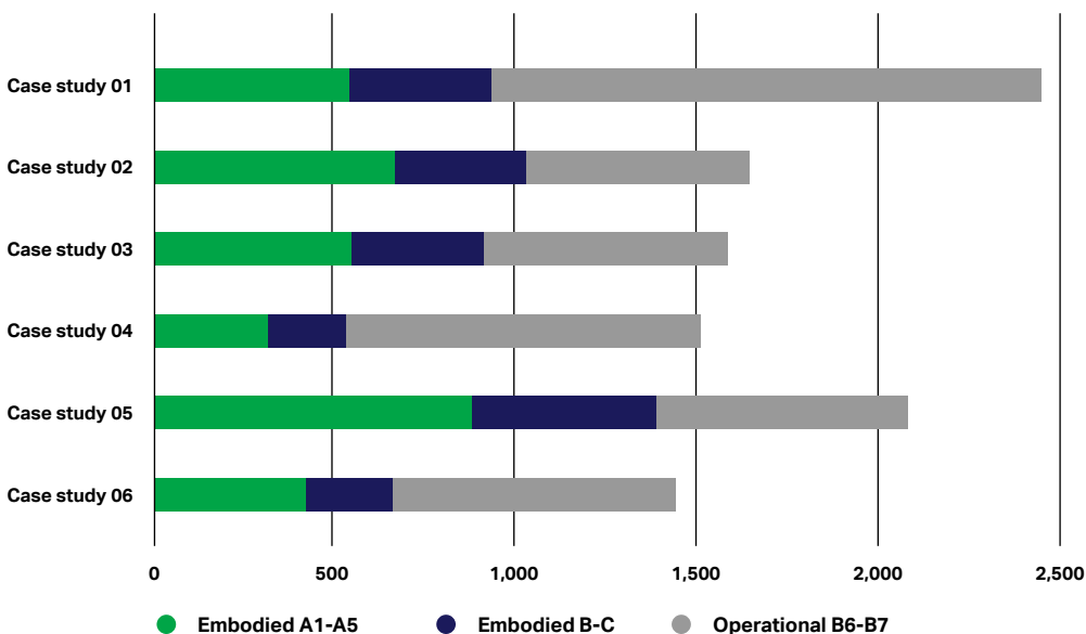
Figure 43: A-C per case study (kgCO 2 e/m 2 )
