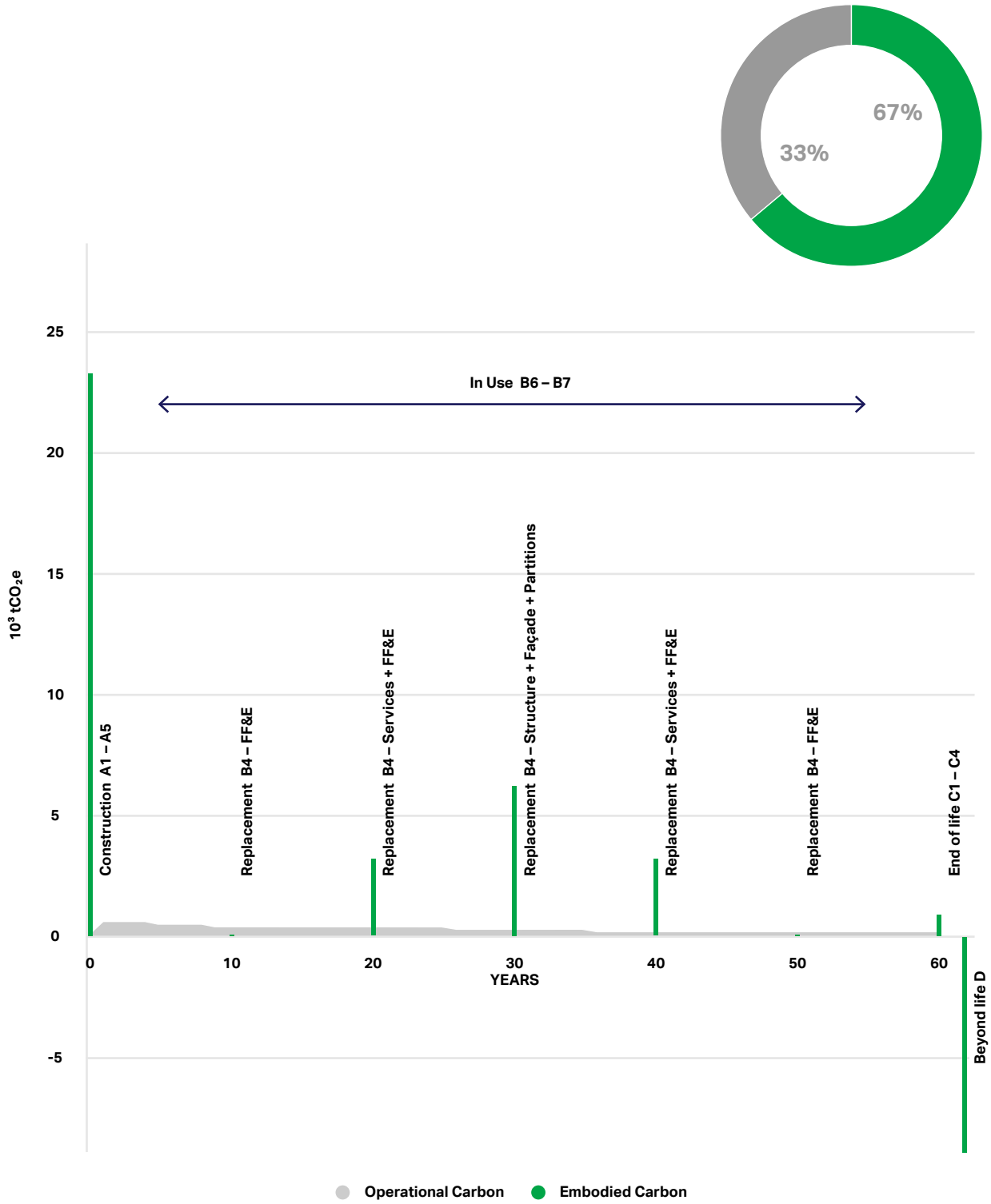
Figure 89: Whole life carbon emissions
