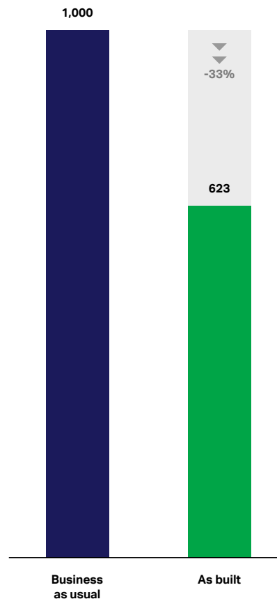
Figure 65: Carbon emissions at practical completion (kgCO 2 e/m 2 GIA)
