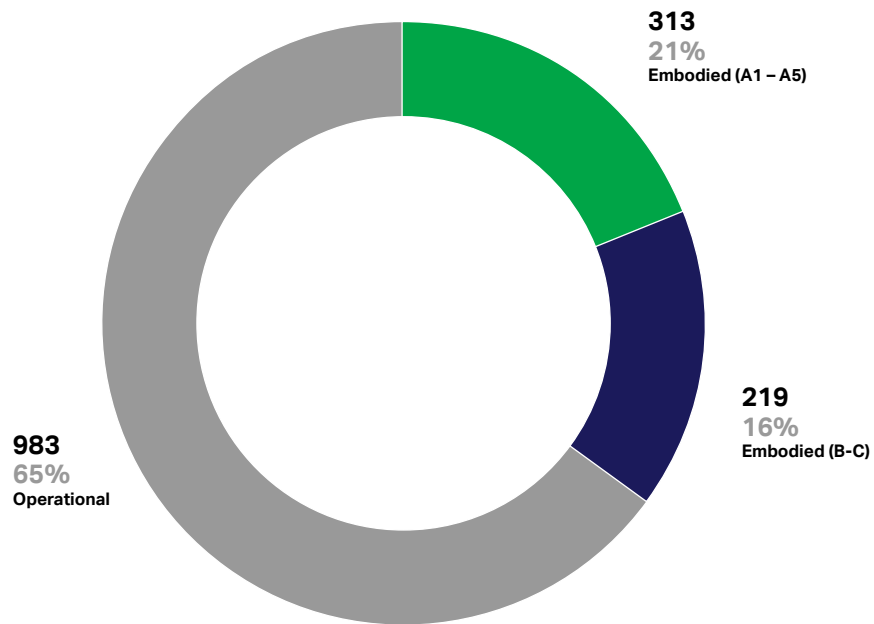
Figure 82: WLCA summary (kgCO 2 e/m 2 )
