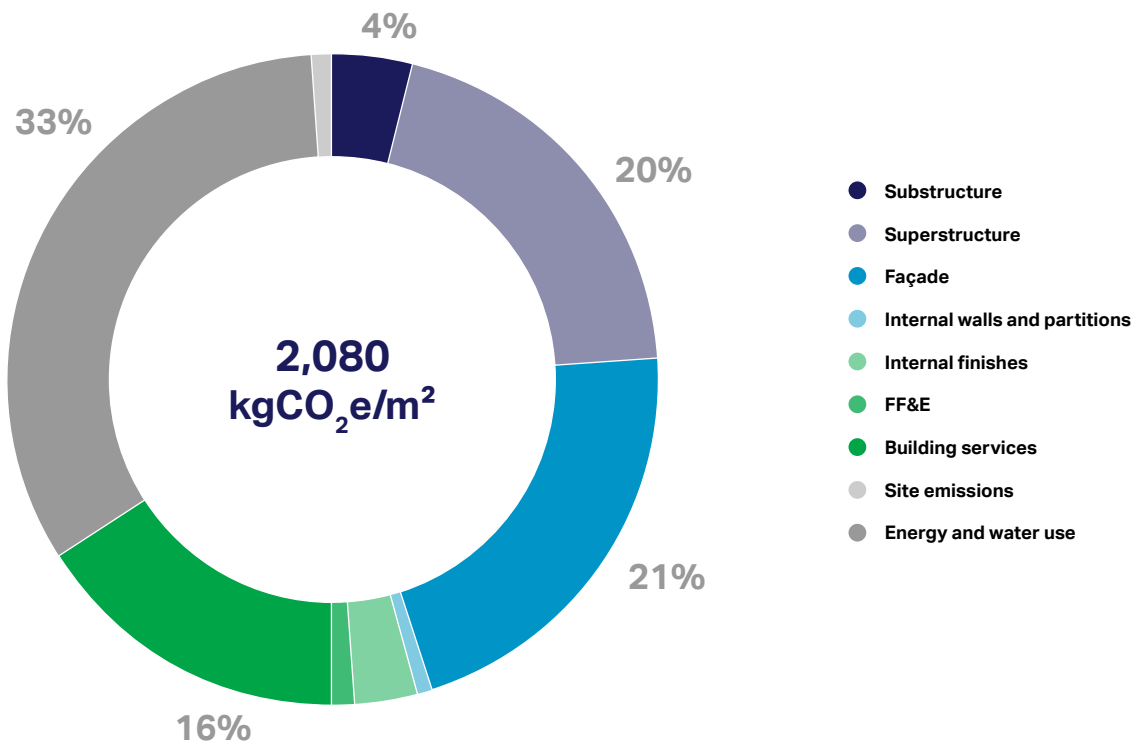
Figure 87: Whole life carbon (A-C)
