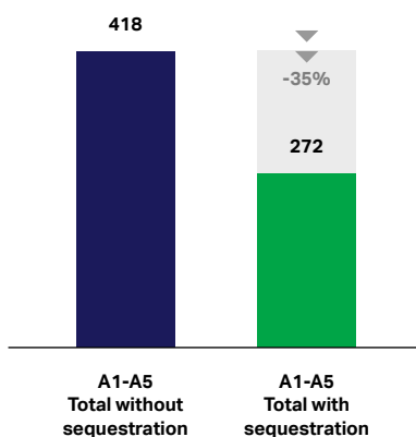
Figure 50: Embodied carbon at practical completion (kgCO 2 e/m 2 )
