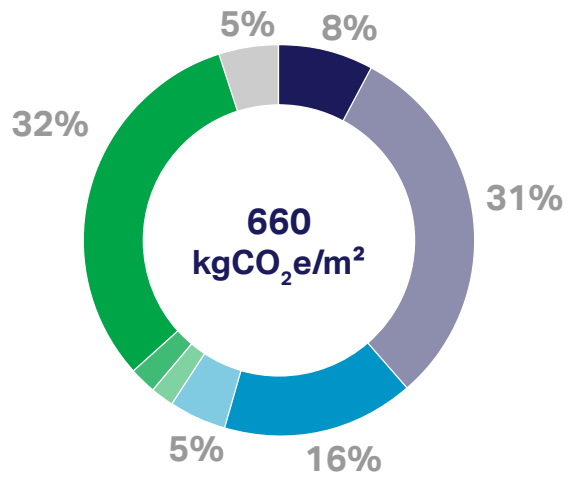
Figure 31: Embodied carbon over the life cycle (A-C)
