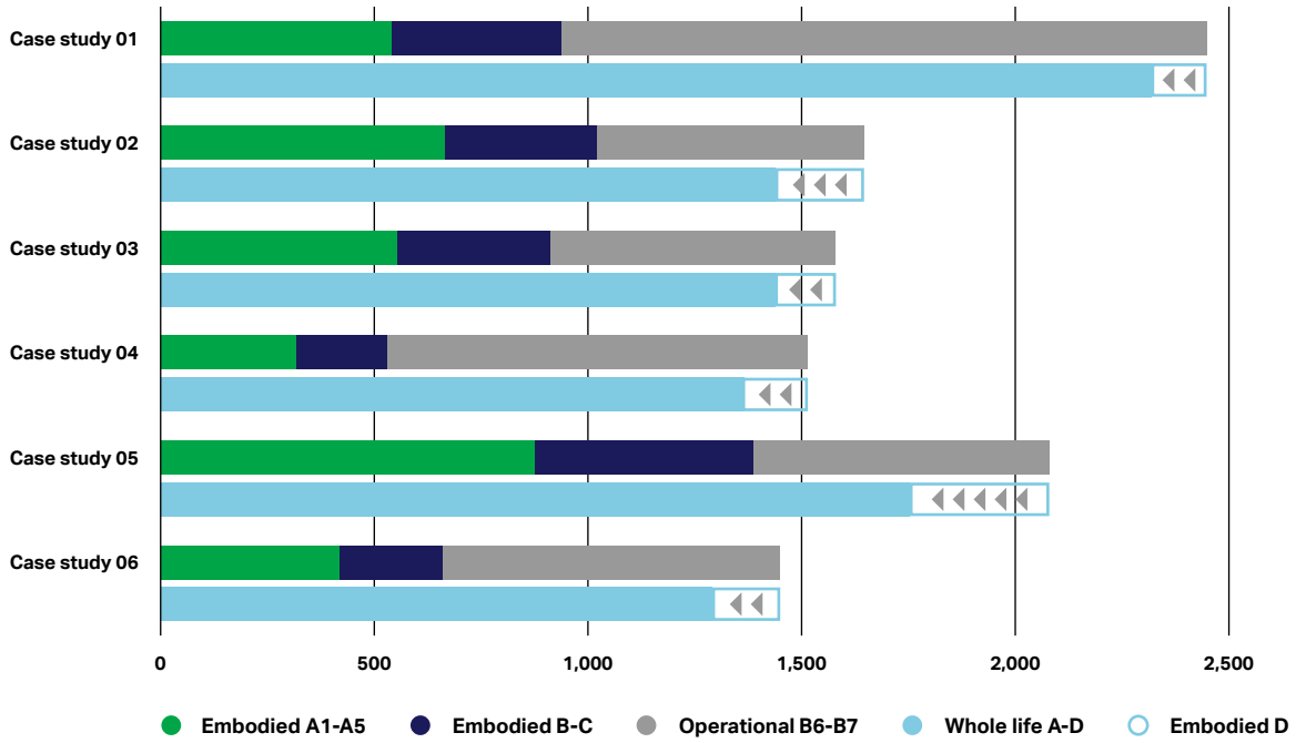
Figure 45: Whole life carbon – A-D (kgCO 2 e / m 2 )
